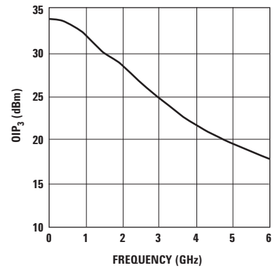
Figure 5. OIP_3 vs. Frequency at I_d = 60 mA.
