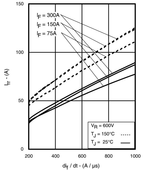
Fig 4. Typical I_{rr} vs. di/dt
